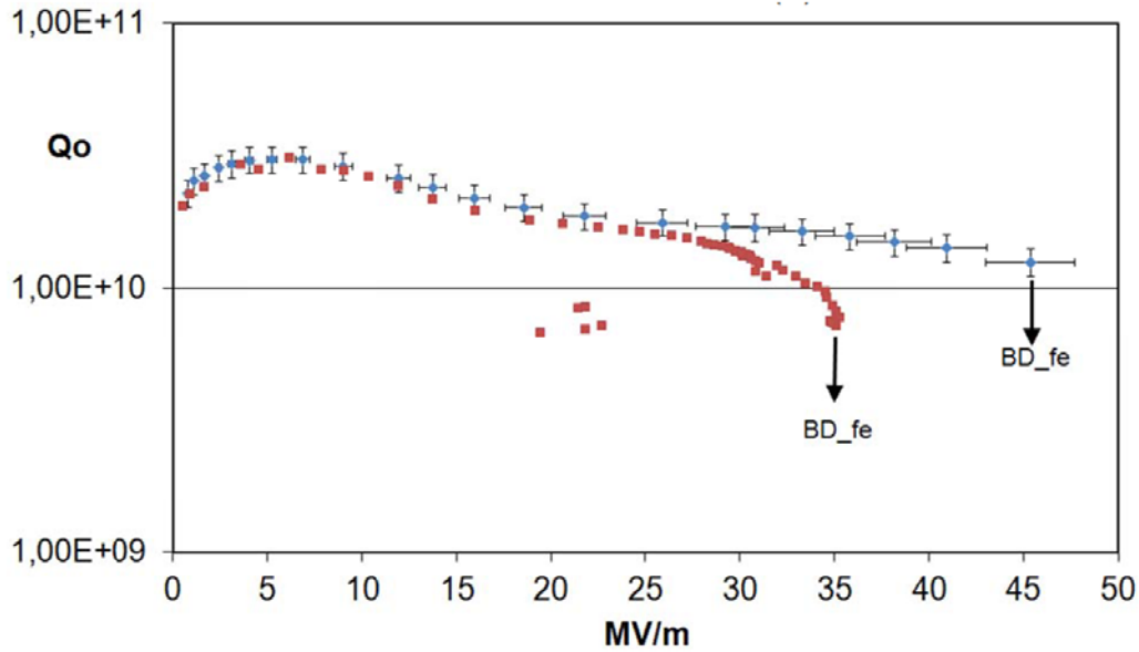
Figure 2: First and final Q_0(E_{acc}) performance of nine-cell cavity AC155 at 2 K after EP treatment. Notice the Q-
